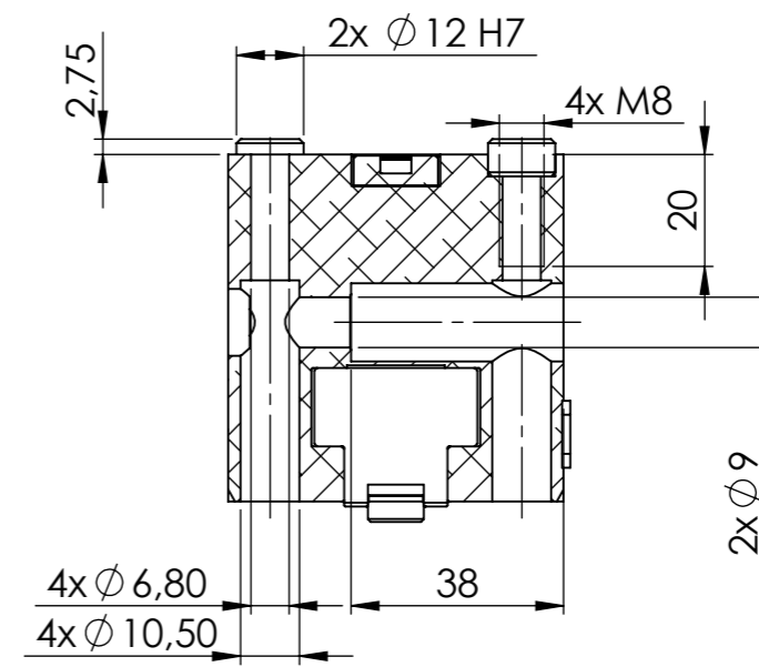
SECTION H-H SCALE 1 : 1.5
